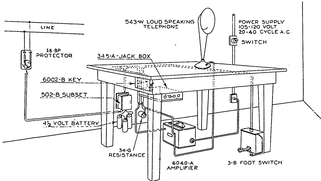
Typical layout for Train Dispatchers equipment.
