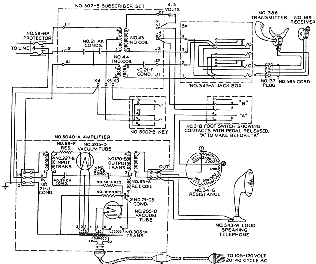
Connection diagram for Train Dispatchers equipment.
